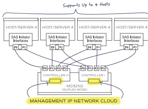
SAS CONFIGURATION
